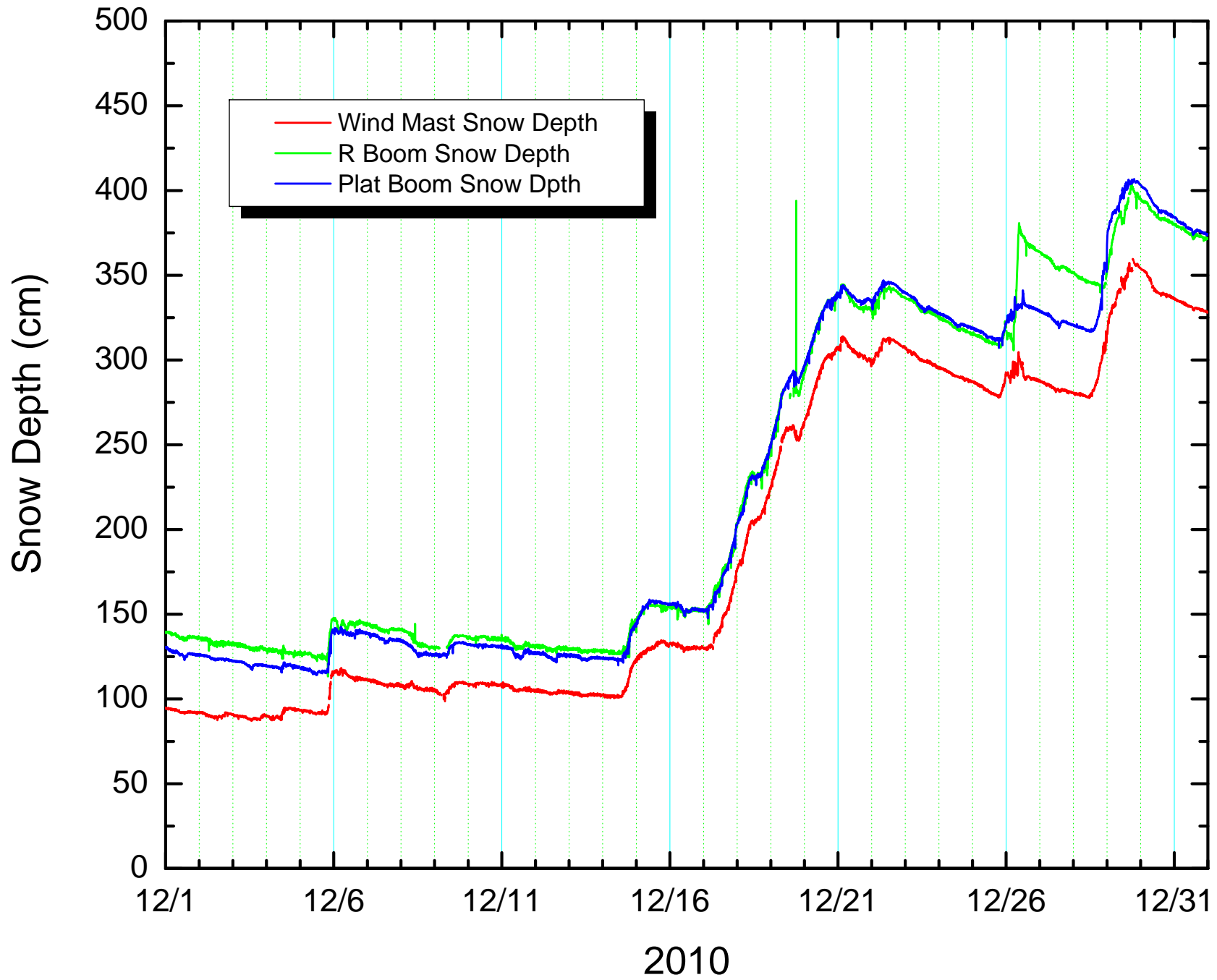
Analyzed Snow Depth
